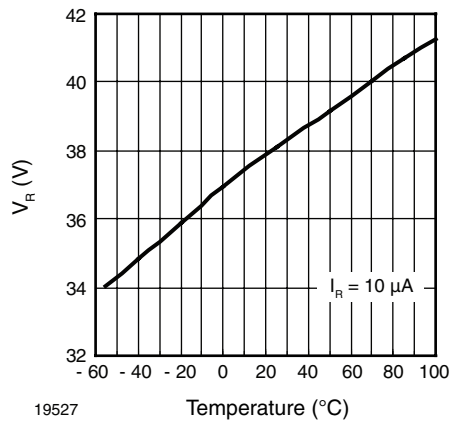
Fig. 3 - Diode Reverse Voltage vs. Temperature
