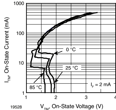
Fig. 5 - Output On Current ( I_{TM} ) vs. Voltage
