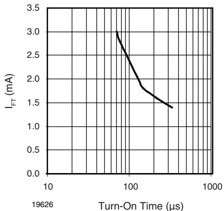
Fig. 8 - Trigger Current vs. Turn-On Time
